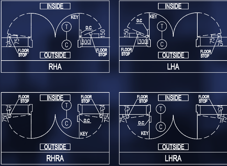
OPENNING DIRECTION AND DOOR CLOSER SIDE STANDARD FLOOR STOP LOCATION
