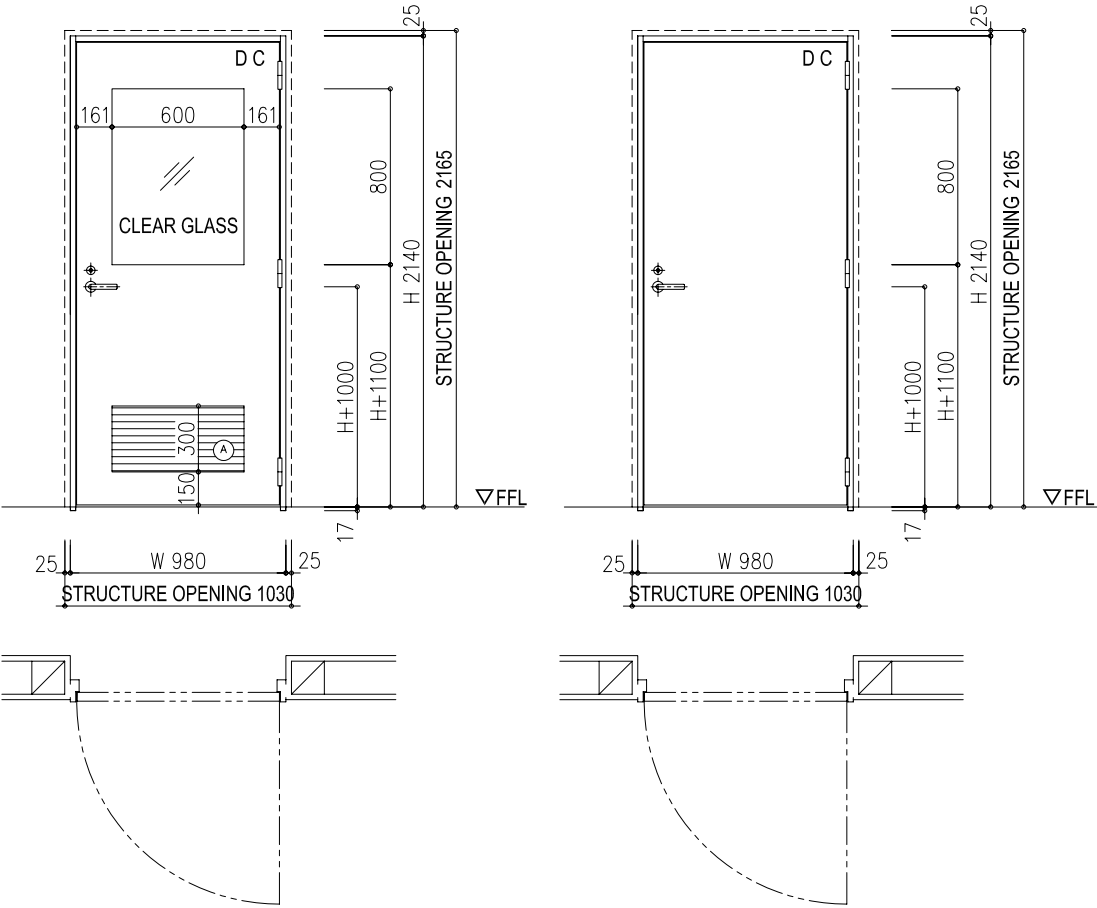
OPENNING DIRECTION AND DOOR CLOSER SIDE STANDARD FLOOR STOP LOCATION
